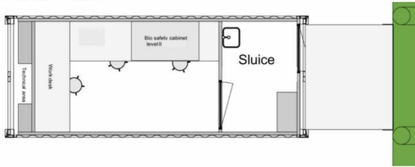
Laboratory Unit Floor Plan
