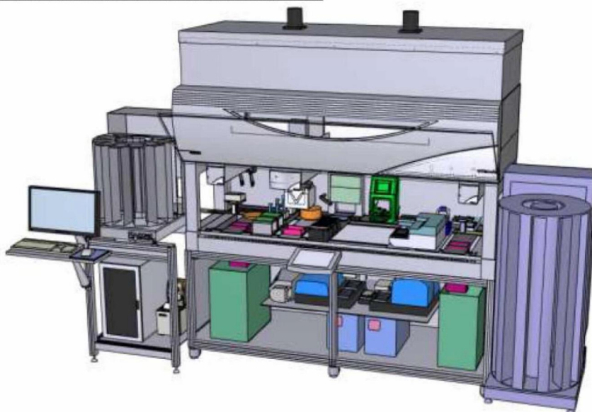
Example picture of the Fluent1080 liquidhandling system with integrated modules
