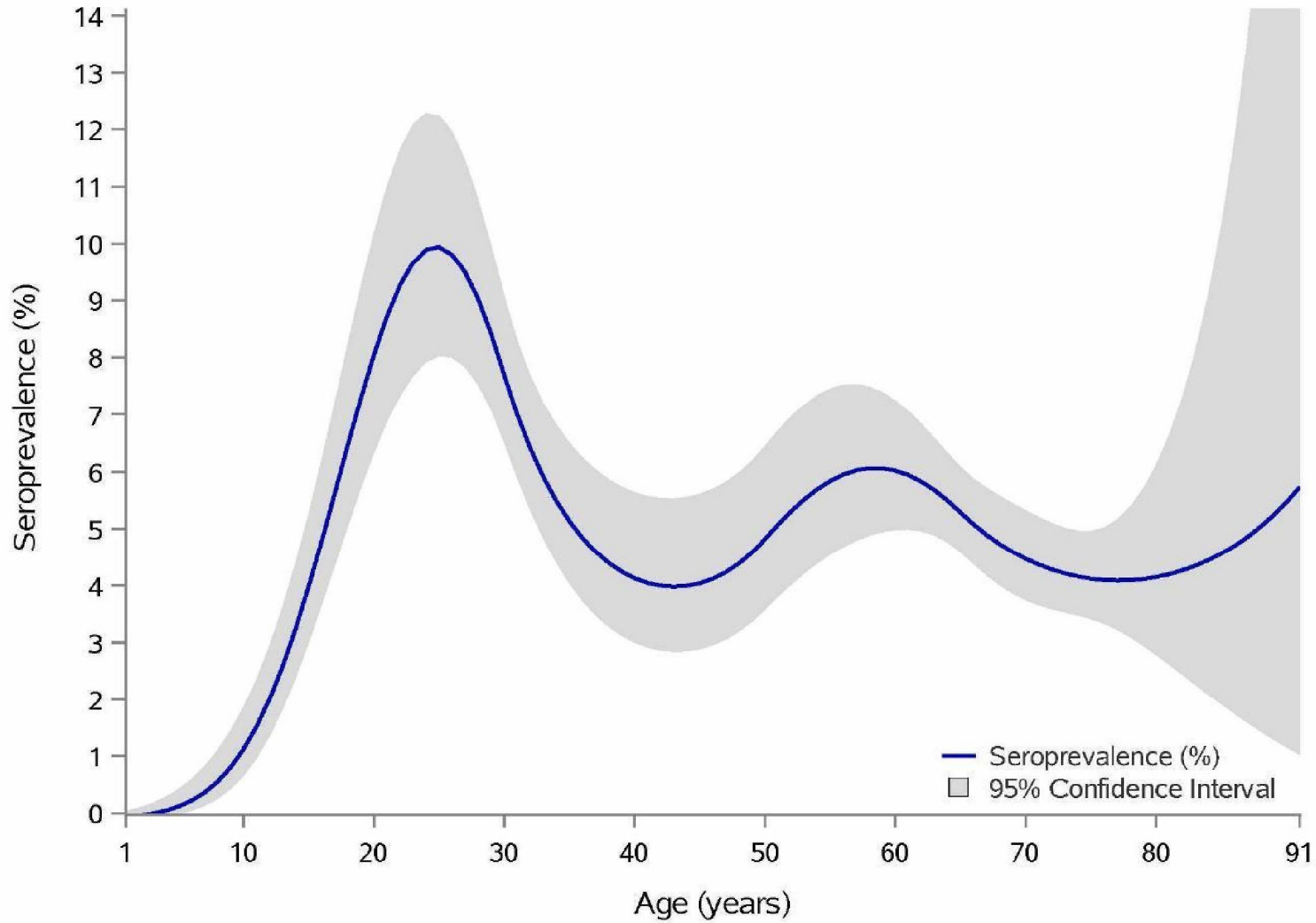
PICO3: SARS-CoV-2 Weighted Seroprevalence in the Netherlands by Age
