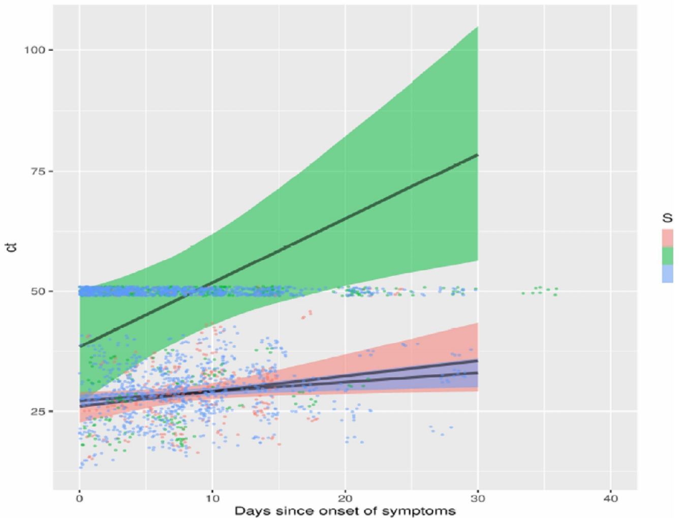
Figure 4. Linear increase of Ct-value in relation to days since onset of symptoms across different disease severity categories. The shaded band indicates 95% Bayesian credible interval. The dots are the original data. Dots positioned at a Ct of 50 or above are censored in the inflated model (i.e. count as either above 50 or a negative individual). Abbreviations: ICU, Intensive Care Unit; OUP, outpatients; WARD, non-ICU hospitalized patients; ct, Ct-value
